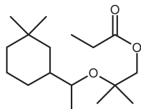
1-Propanol, 2-[1-(3,3-dimethyl-cyclohexyl)ethoxy]-2-methyl-,propanoate
